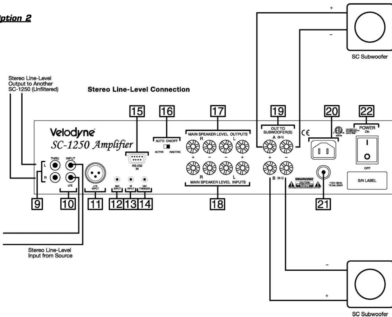
Figure 3B: Stereo Line-Level Connection.
